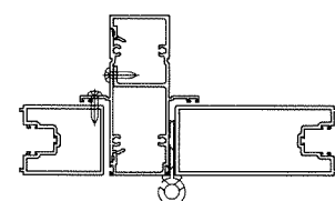
UNREINFORCED
